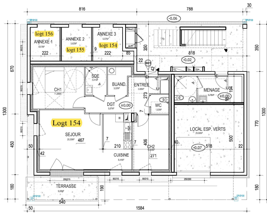
BATIMENT G PLAN RDC 1/100
