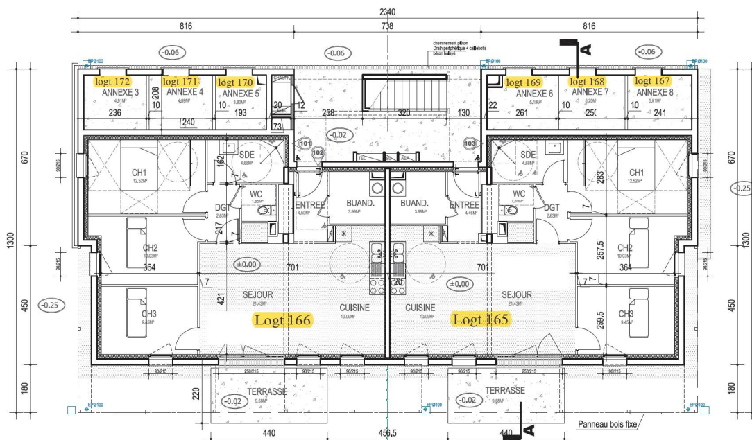
PLAN R+1 1/100
