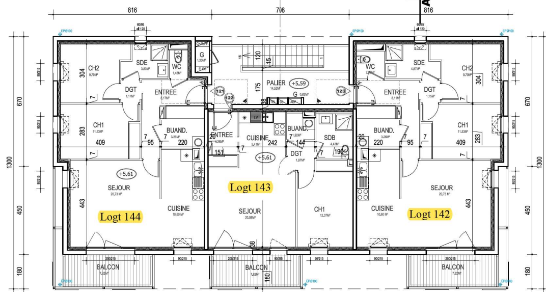
PLAN R+2 1/100
