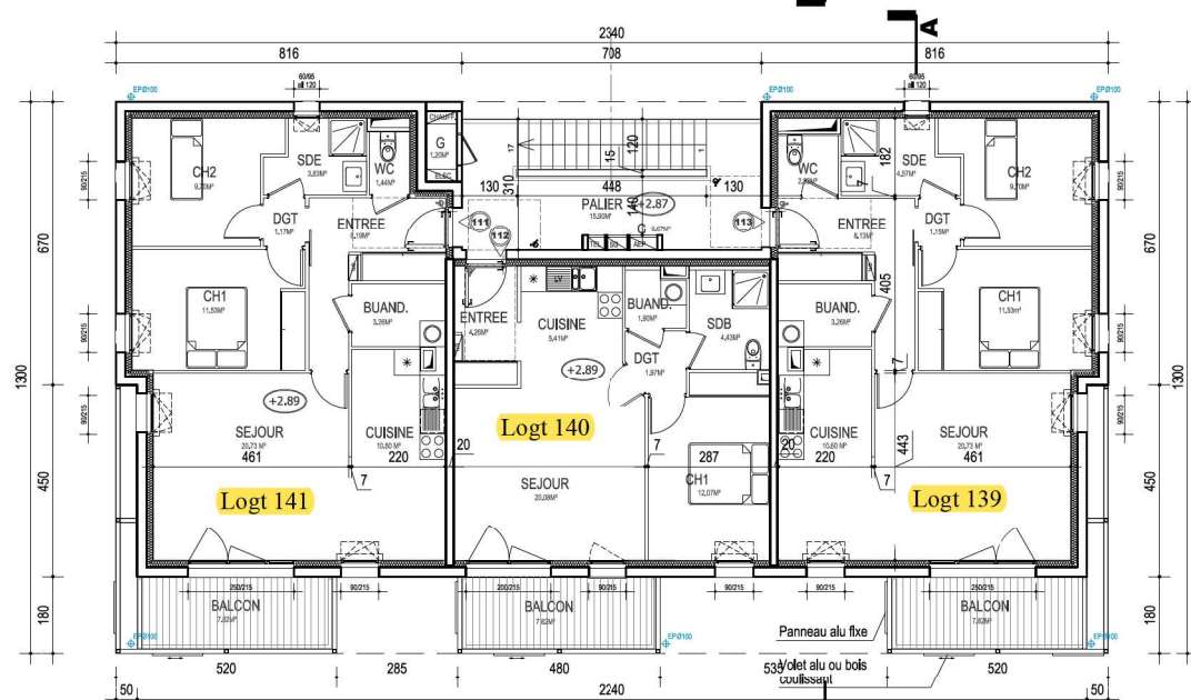
PLAN R+1 1/100
