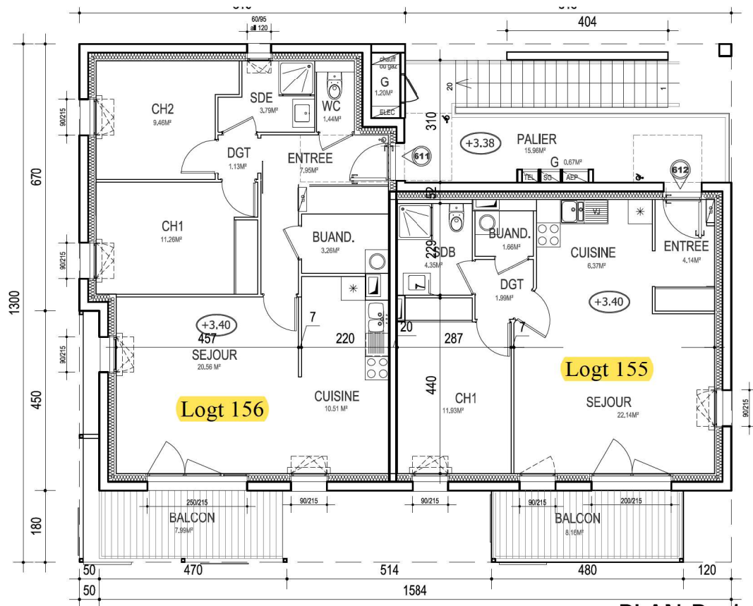
PLAN R+1 1/100
