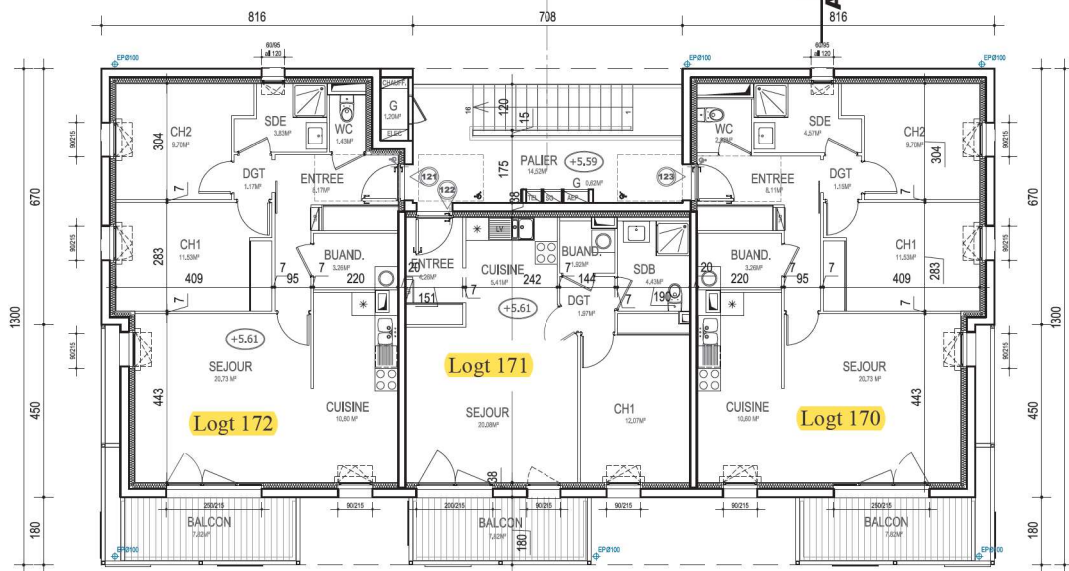
PLAN R+2 1/100
