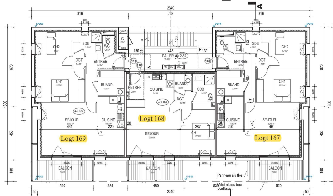
PLAN R+1 1/100
